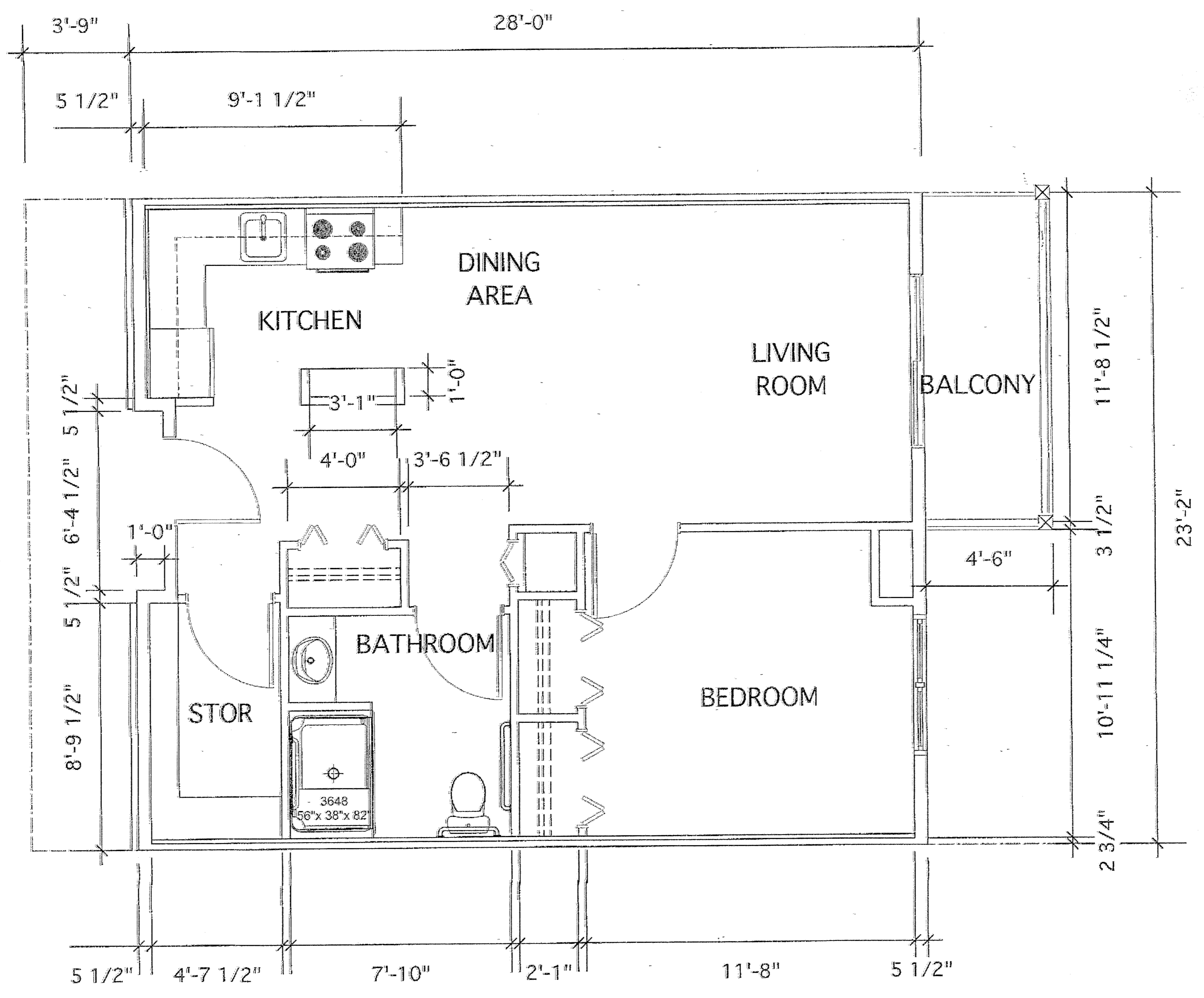
2 303 TYPE-B UNIT - ONE BEDROOM (4 UNITS TOTAL) 1/4" = 1'-0"
